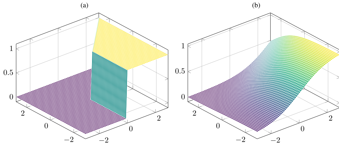
Figure 4: (a) Single output of an \text{arg max} function. The derivative is null almost everywhere, i.e. there is no descent direction. (b) Single output of the differentiable relaxation. The derivatives are non-null.
